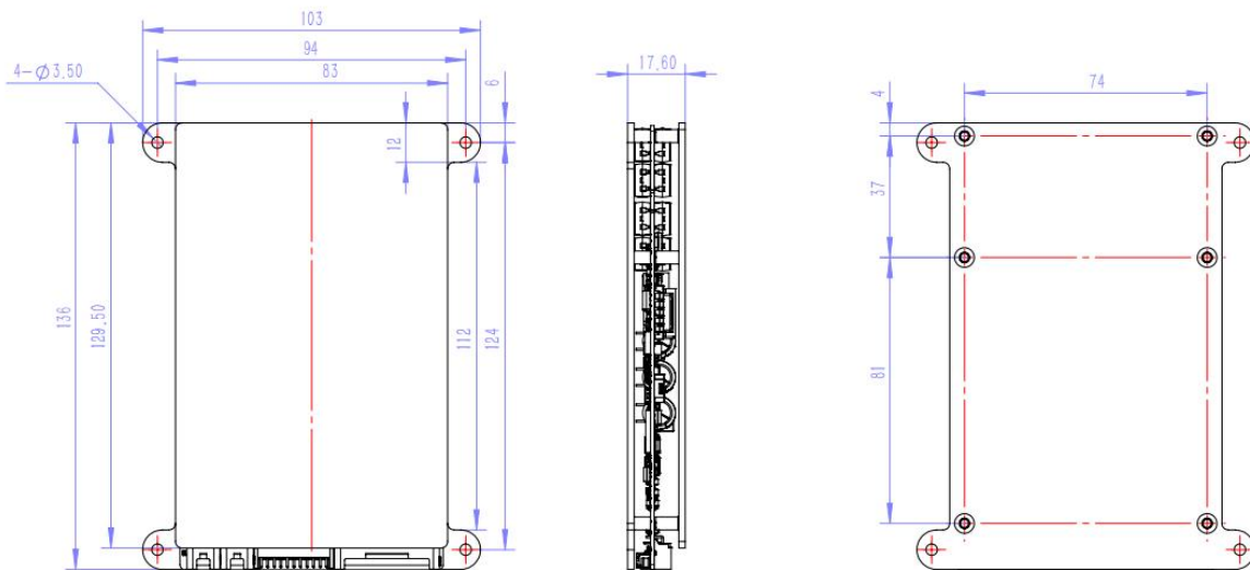
JK-BD6AxxS-6P/8P外形尺寸
